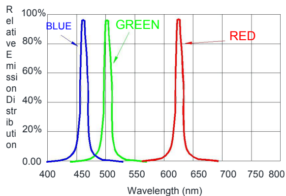
Wavelength Characteristics
